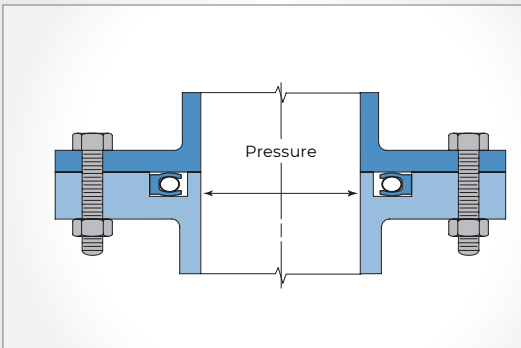
STATIC INSIDE FACE SEAL
