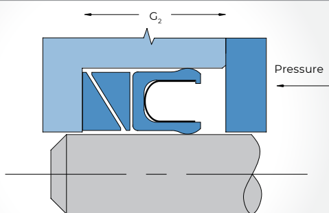
GLAND WIDTH FOR STANDARD OMNISEAL® SEAL PLUS BACK-UP RING
