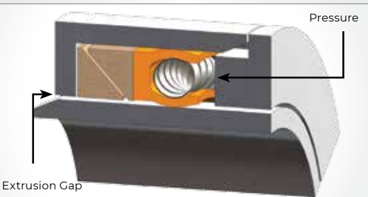
ROD SEAL INSTALLATION WITH DUAL BACK-UP RINGS
