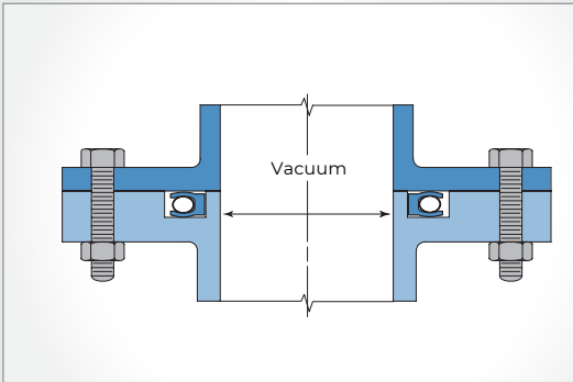
STATIC OUTSIDE FACE SEAL
