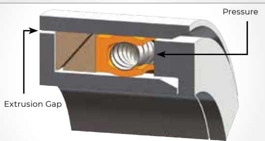
PISTON SEAL INSTALLATION WITH DUAL BACK-UP RINGS
