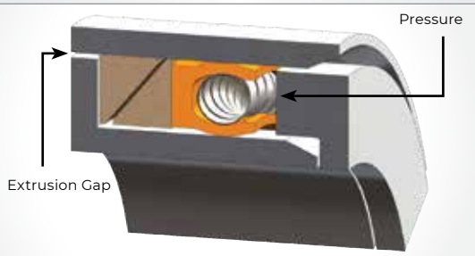
PISTON SEAL INSTALLATION WITH DUAL BACK-UP RINGS
