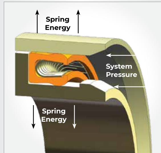
Omniseal® 400A seal in working conditions
