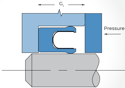
GLAND WIDTH FOR EXTENDED HEEL OMNISEAL® SEAL
