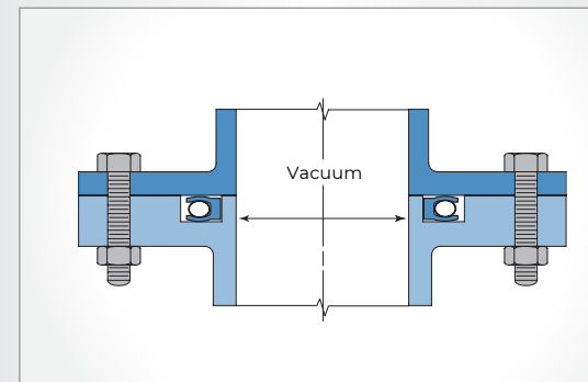
STATIC OUTSIDE FACE SEAL
