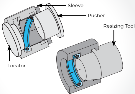
Installation of Omniseal® APS seal in closed rod gland (left); Completion of installation (right)
