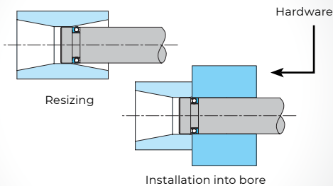
Resized (left); Installation into bore (right)
