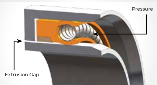
HIGH MODULUS ANTI-EXTRUSION/WEAR RING
