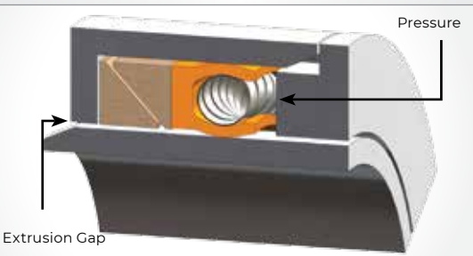
ROD SEAL INSTALLATION WITH DUAL BACK-UP RINGS
