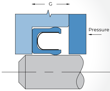
GLAND WIDTH FOR STANDARD OMNISEAL® SEAL
