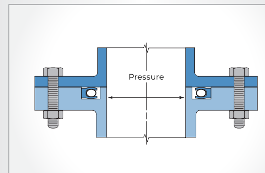
STATIC INSIDE FACE SEAL
