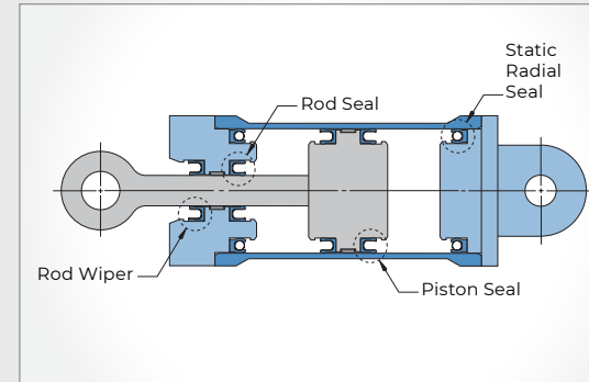
DYNAMIC RADIAL SEAL
